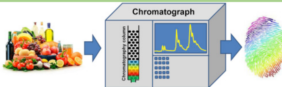
Figure 2: Chromatographic Fingerprinting 17
